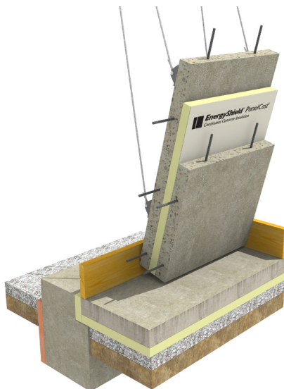
SITE-CAST TILT-UP
