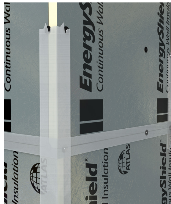
Figure 5: Apply joint sealing product at joints and all inside and outside corners, extending at least 2" on the face of board.
